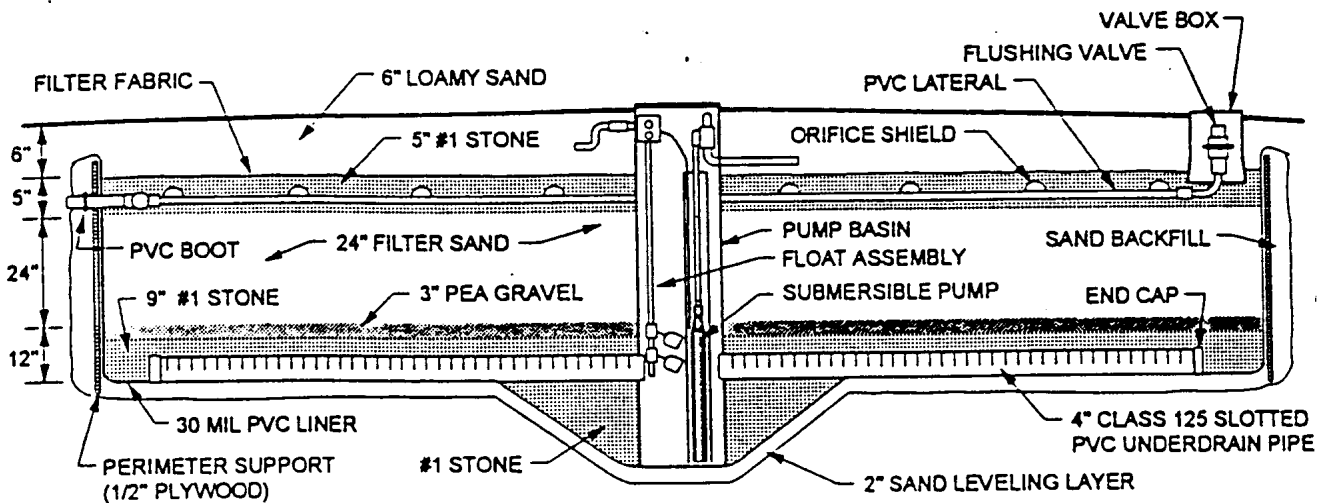
Fig. 14. Cross section of a single pass sand filter showing an internal pump chamber. Units
