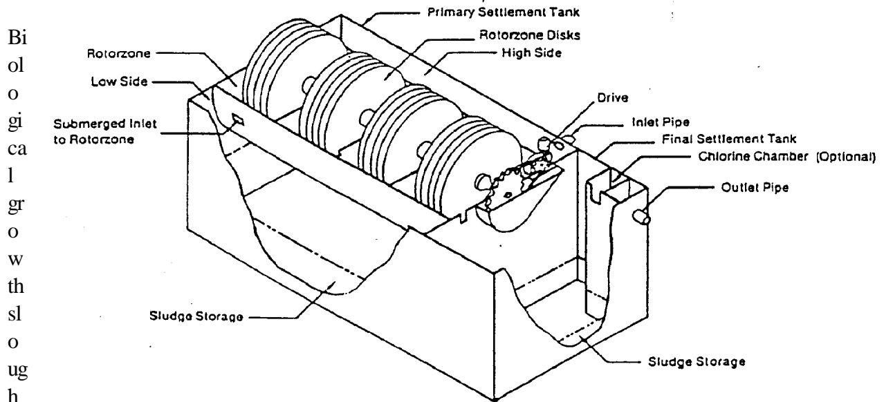
Fig. 13. Schematic of a rotating biological contactor (CSM Rotodisk Inc.)
